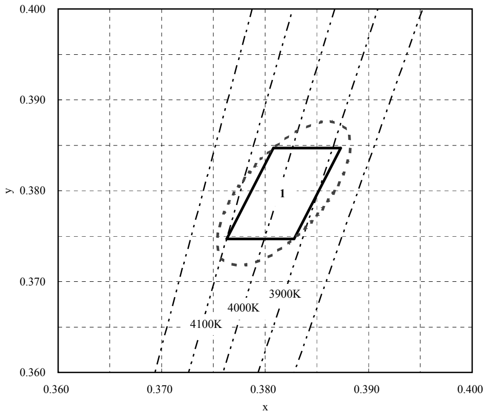
Chromaticity Diagram
